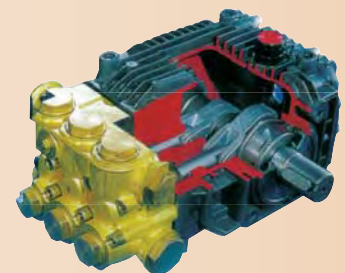
Piston Pump
